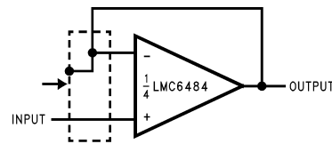
Follower
